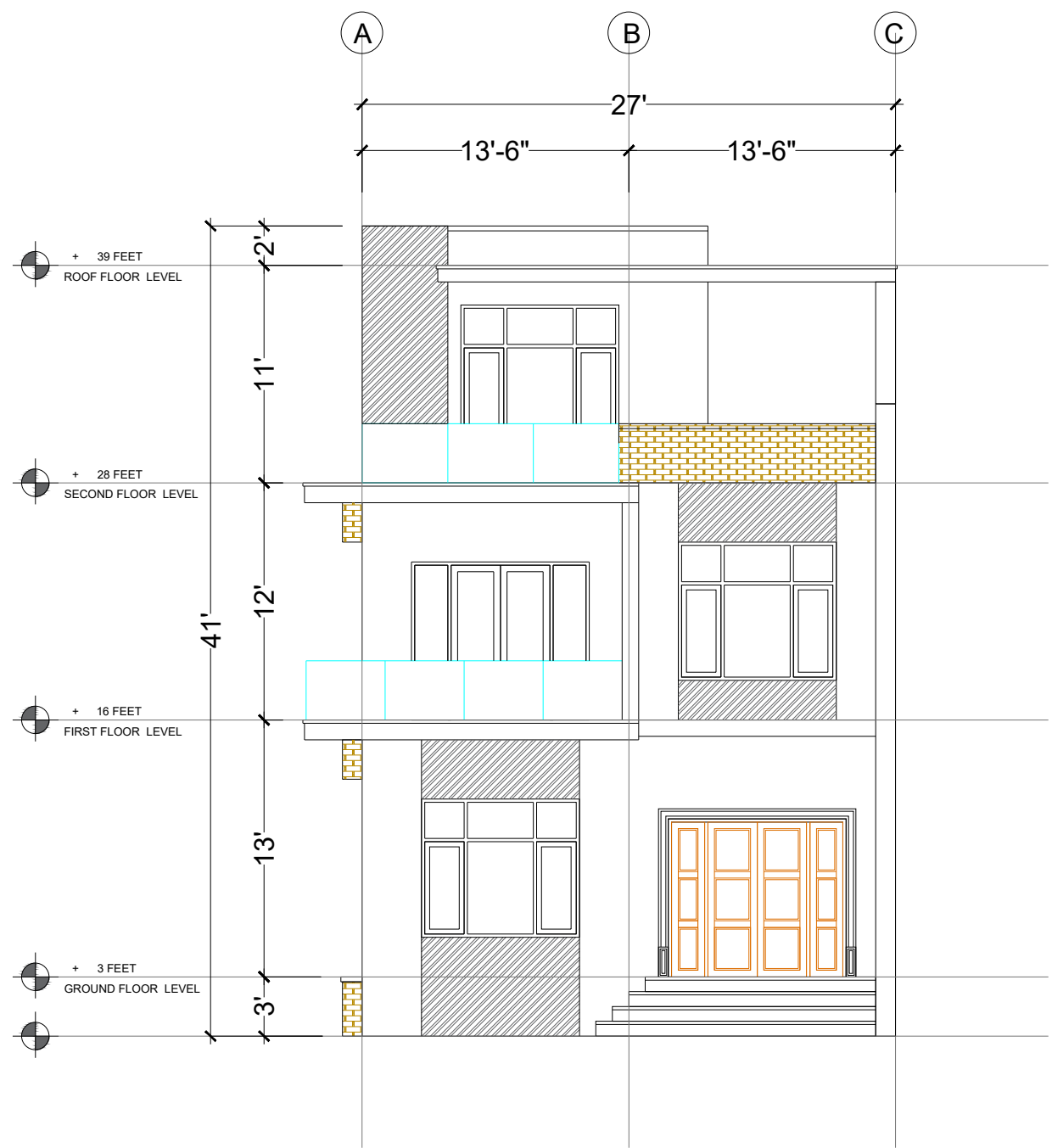
ELEVATION-1
