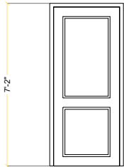
elevation DOOR-5
