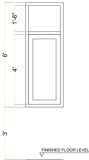
elevation WINDOW-1 2' 2" X 6' Alu: & Glass
