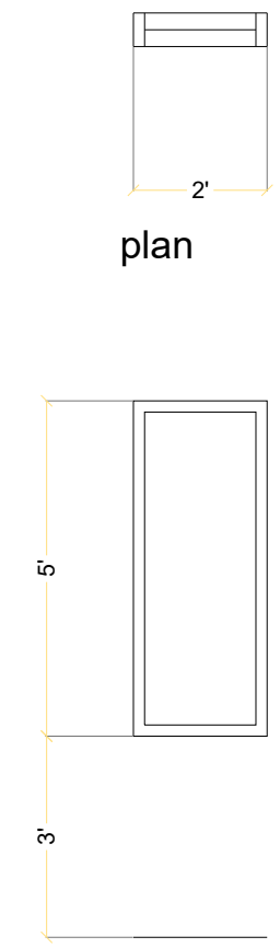
elevation GLASS PANEL-2 2' X 5' Alu: & Glass WINDOW 1,2,3
