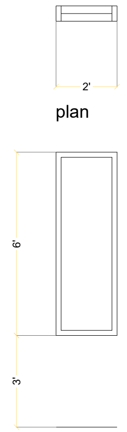
elevation GLASS PANEL-2 2' X 6' Alu: & Glass
