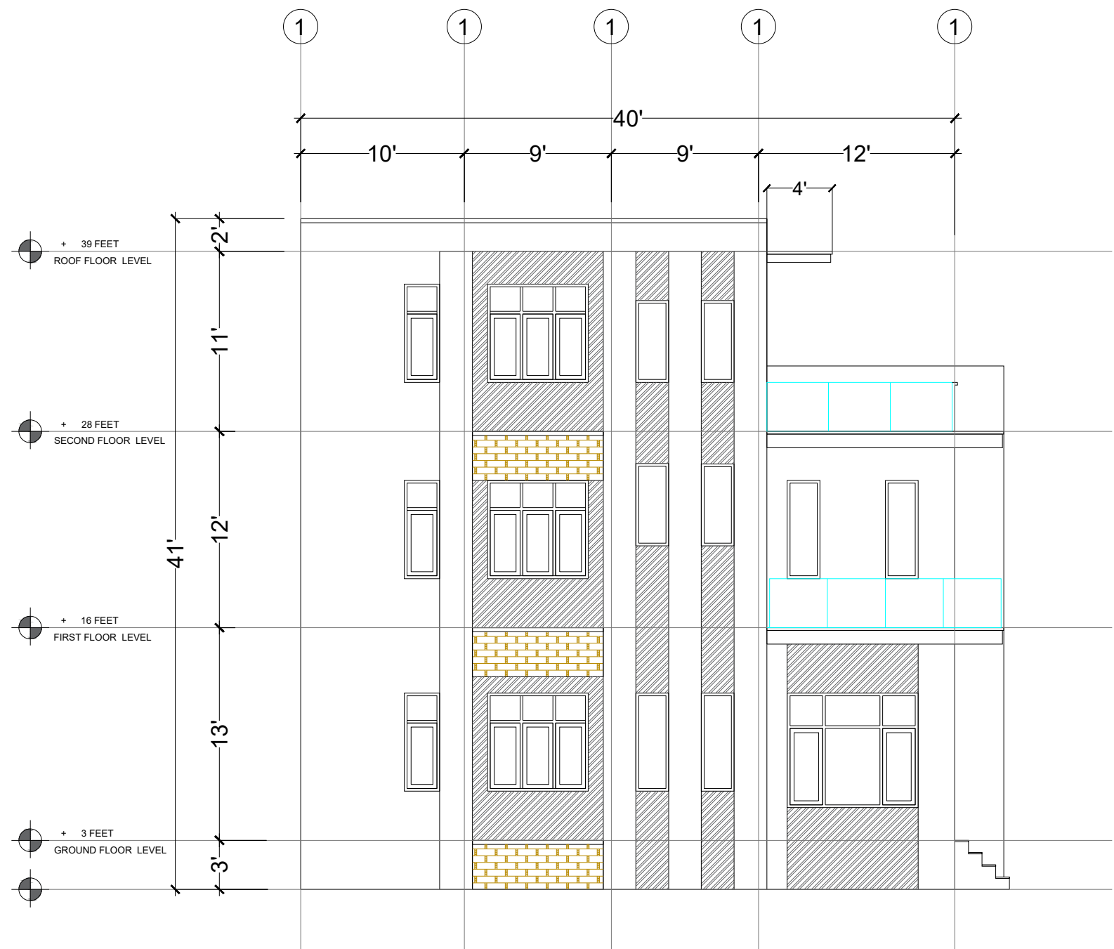
ELEVATION-2
