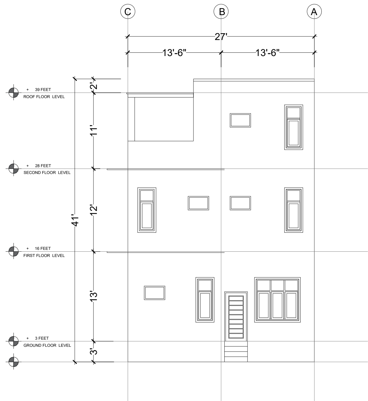
ELEVATION-3
