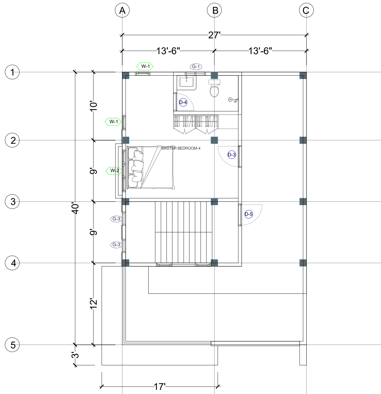
ROOF FLOOR PLAN
