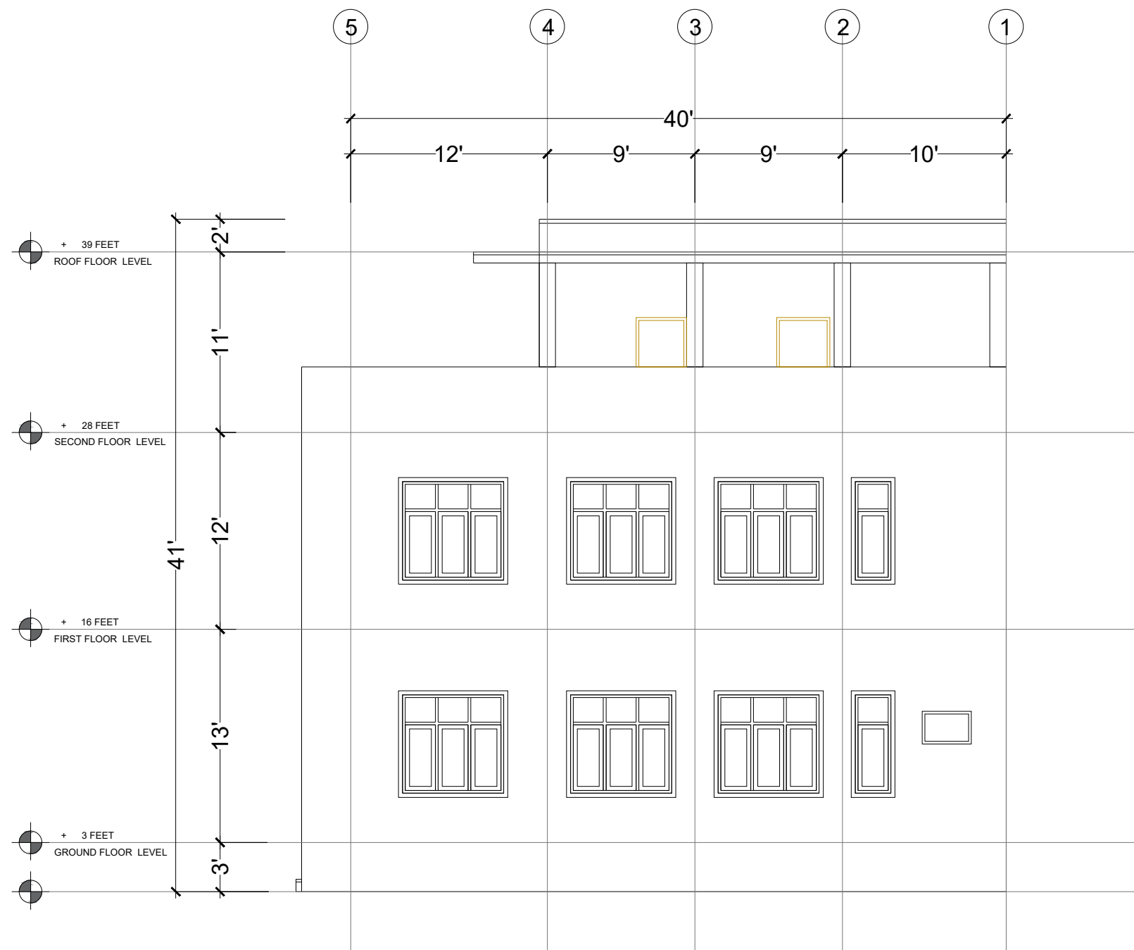
ELEVATION-4
