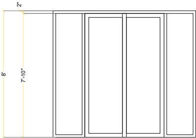
elevation DOOR-2
