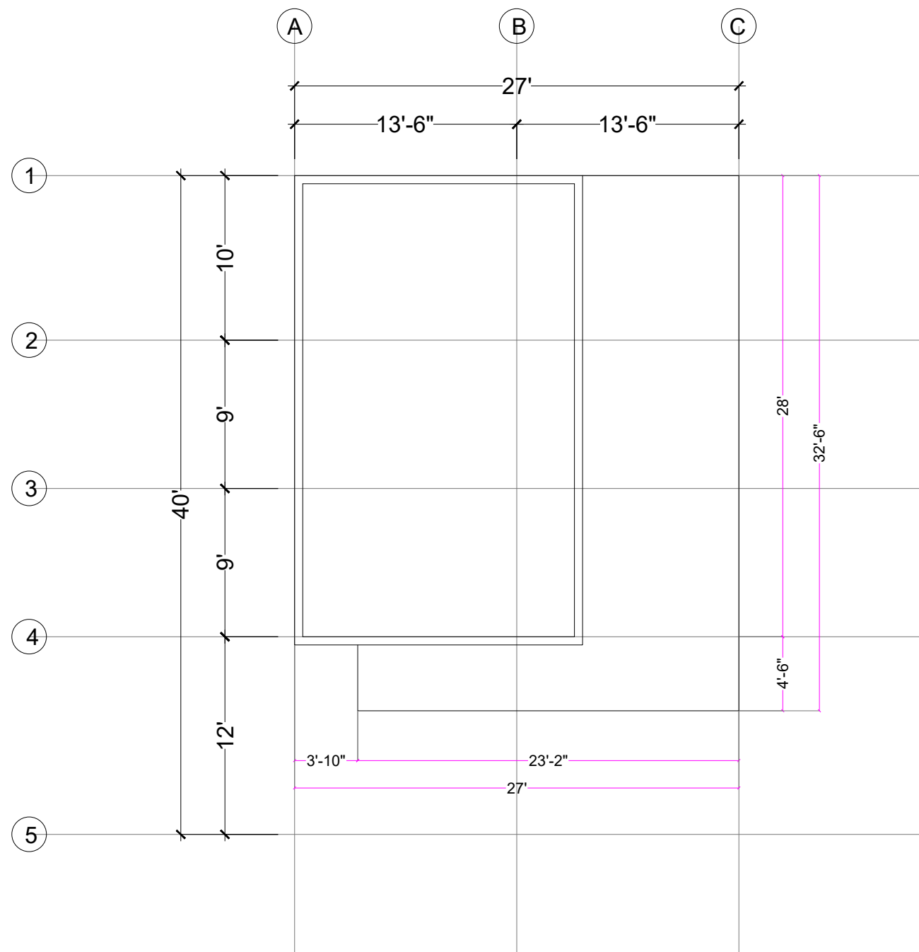
ROOF TOP PLAN
