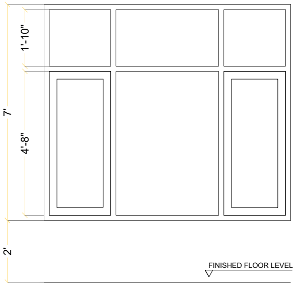
elevation WINDOW-3 8' X 7' Alu: & Glass
