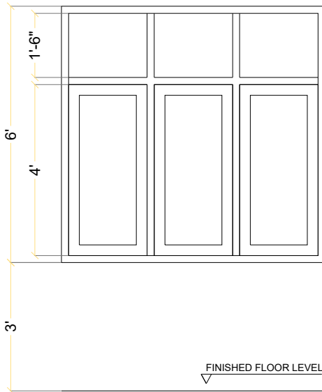
elevation WINDOW-2 6' 2" X 6' Alu: & Glass
